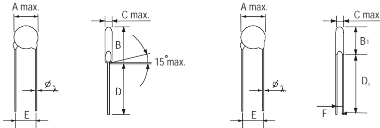
KINKED LEAD TYPE Dimension Table
